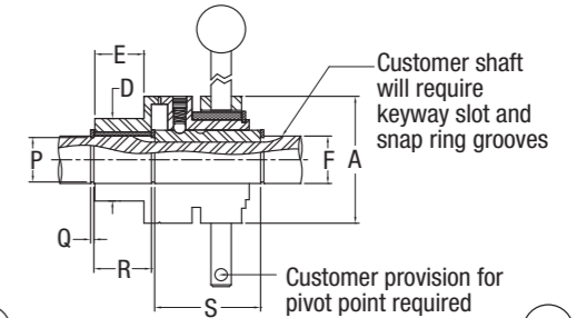
JK KIT - LESS SHAFT
