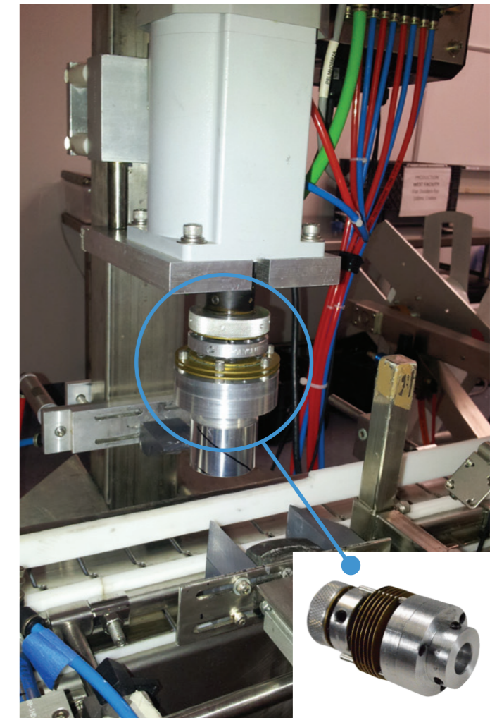
Capping - The V-Series slipper is the ideal solution for torque control on capping machines.
