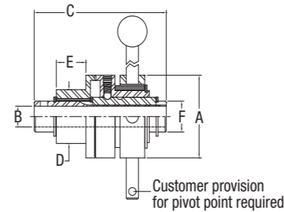
JH CLUTCH - WITH HUB
