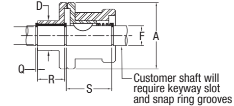
DK KIT - LESS SHAFT
