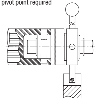
Engage and disengage mechanism Drive roll adapted to housing
