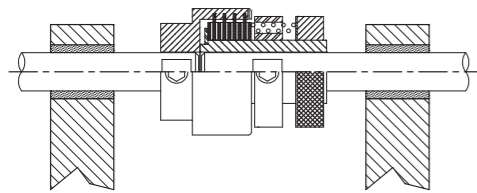
FIG. 1 Shaft to Shaft. Shafts must be supported and aligned within .010" - .015".
