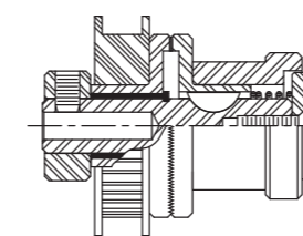
Phase adjustment shaft to pulley Pulley pressed onto knurled housing
