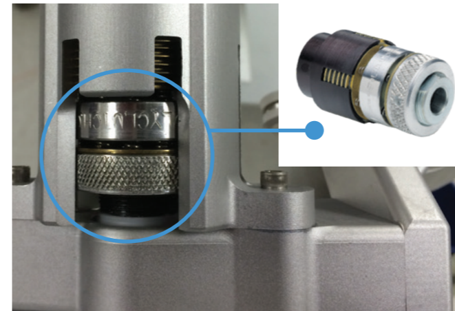
Surgical Device - A Slip-Ease clutch is used as a retention hinge on a mounting platform.
