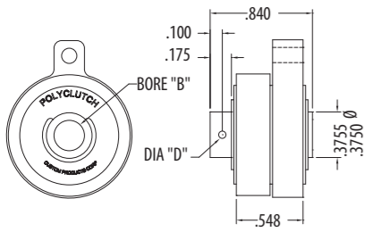
Duplex Assembly all Combinations Available Shown with HEO and HEA Single Assemblies Model HEOA
