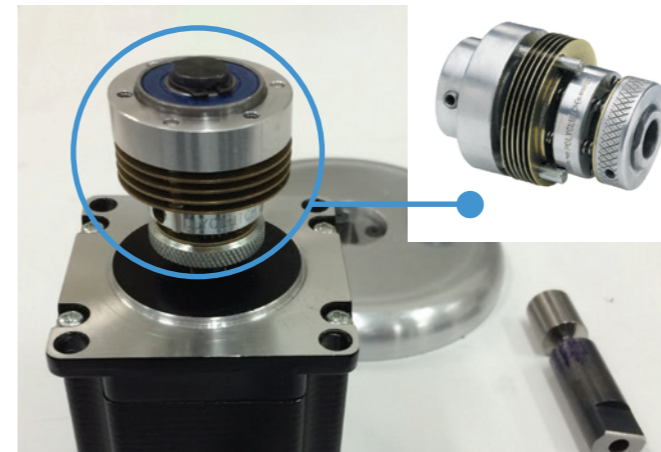
Dental Tool - The Polyclutch® slipper provides precision torque control during the manufacturing of dental implants.
