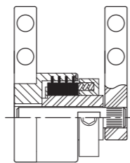
FIG. 8 Rotary position holder (hinge).
