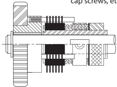
FIG. 4 Gear/Pulley/Sprocket modified with pins for engagement. Housing is eliminated.
