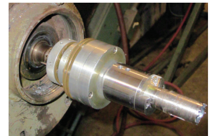
Mechanical Safety - The V-Series Slipper provides overload protection and increases operator safety to this manual cutting tool. This mechanical slip clutch limits the amount of torque that is transferred to the cutting tool, making this a safer operation for the user.
