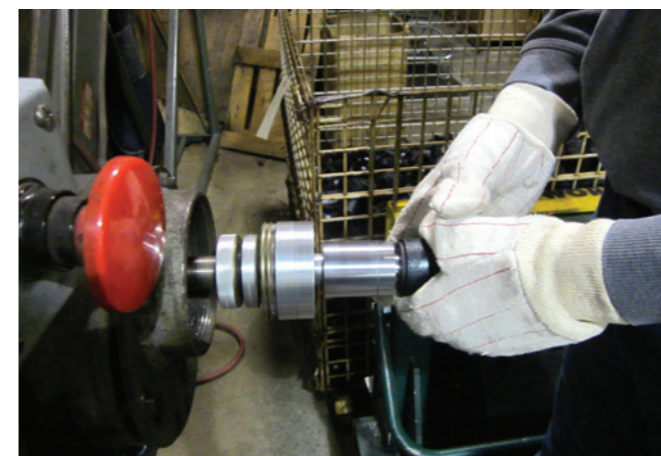
Mechanical Safety - The V-Series Slipper provides overload protection and increases operator safety to this manual cutting tool. This mechanical slip clutch limits the amount of torque that is transferred to the cutting tool, making this a safer operation for the user.
