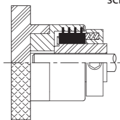
FIG. 6 Knob adapted to housing knurl, set screw, pin, etc.
