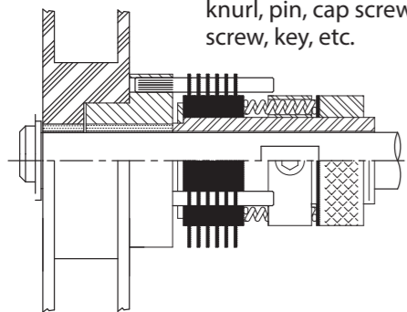
FIG. 5 Gear/Pulley/Sprocket integrated as part of cartridge.
