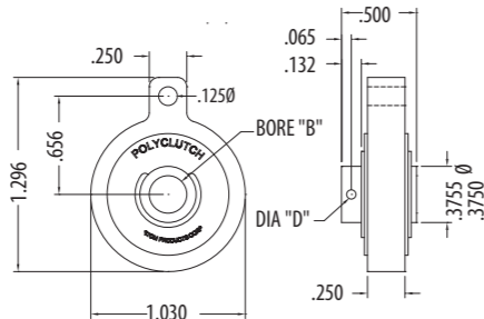
Single Assembly Model HEA Solid Arm
